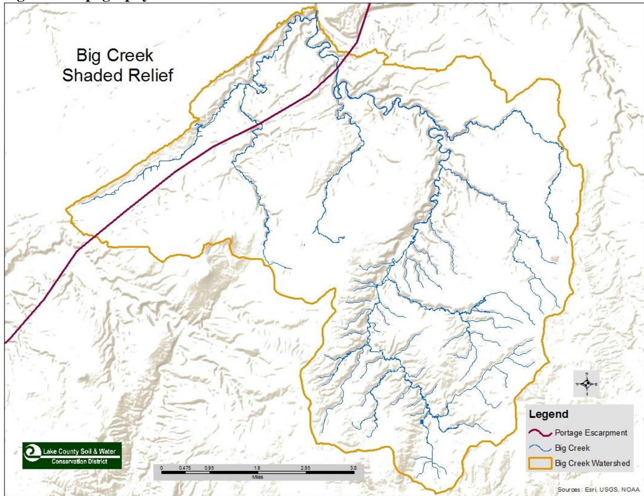
Figure 6. Topography- Shaded Relief
