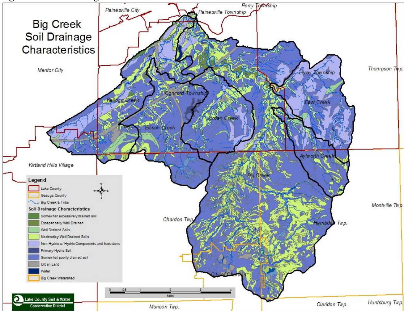
Figure 11. Soil Drainage Characteristics
