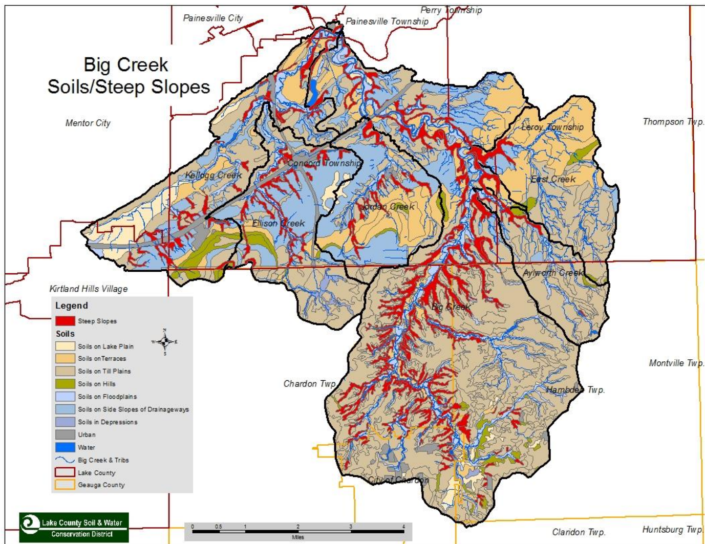
Figure 10. Soils with Steep Slopes
