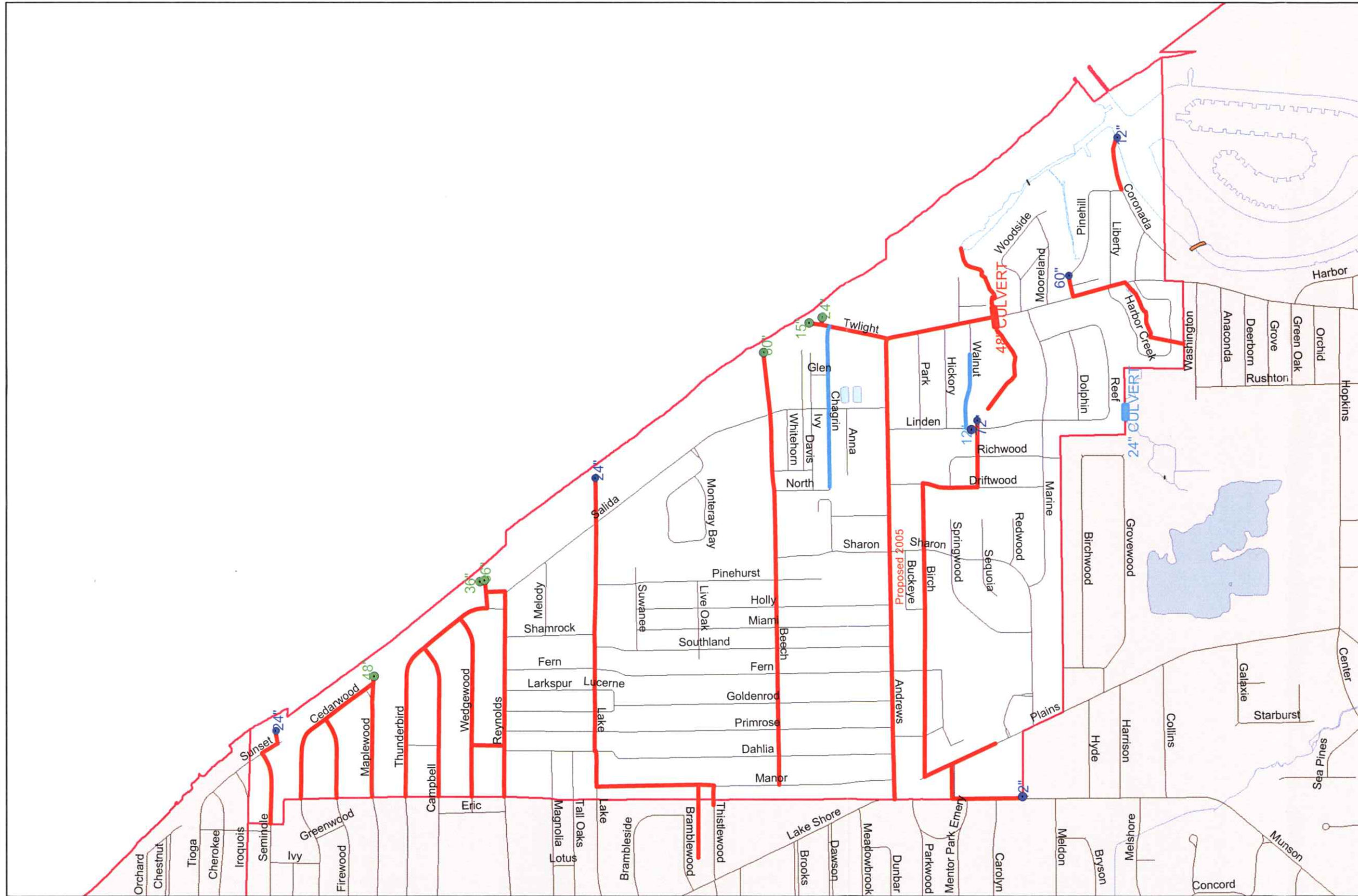
GENERAL PLAN OF DRAINAGE FIGURE 6-23 MENTOR ON THE LAKE
