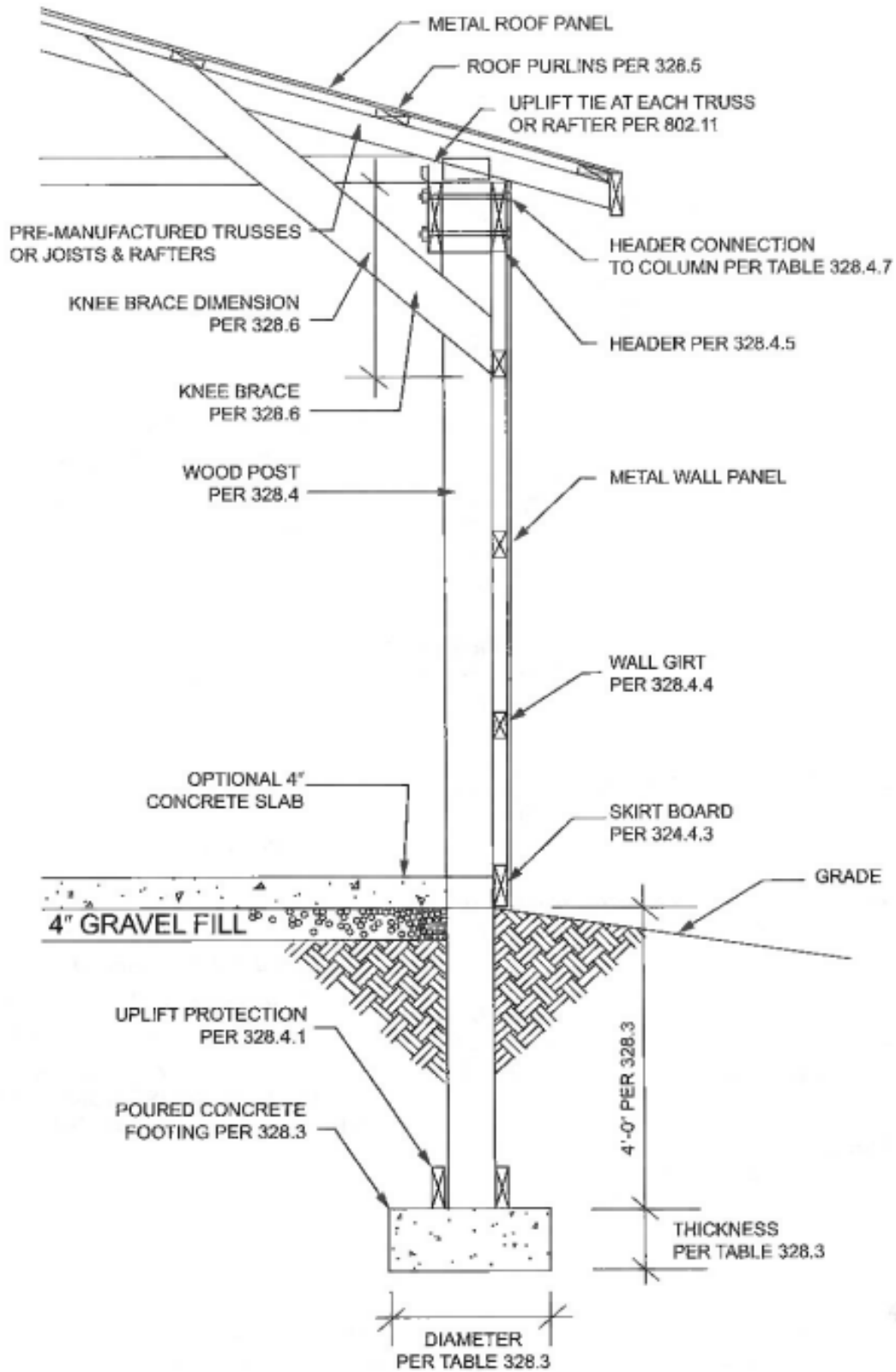
FIGURE 328 POST AND FRAME WALL SECTION (NO SCALE)
